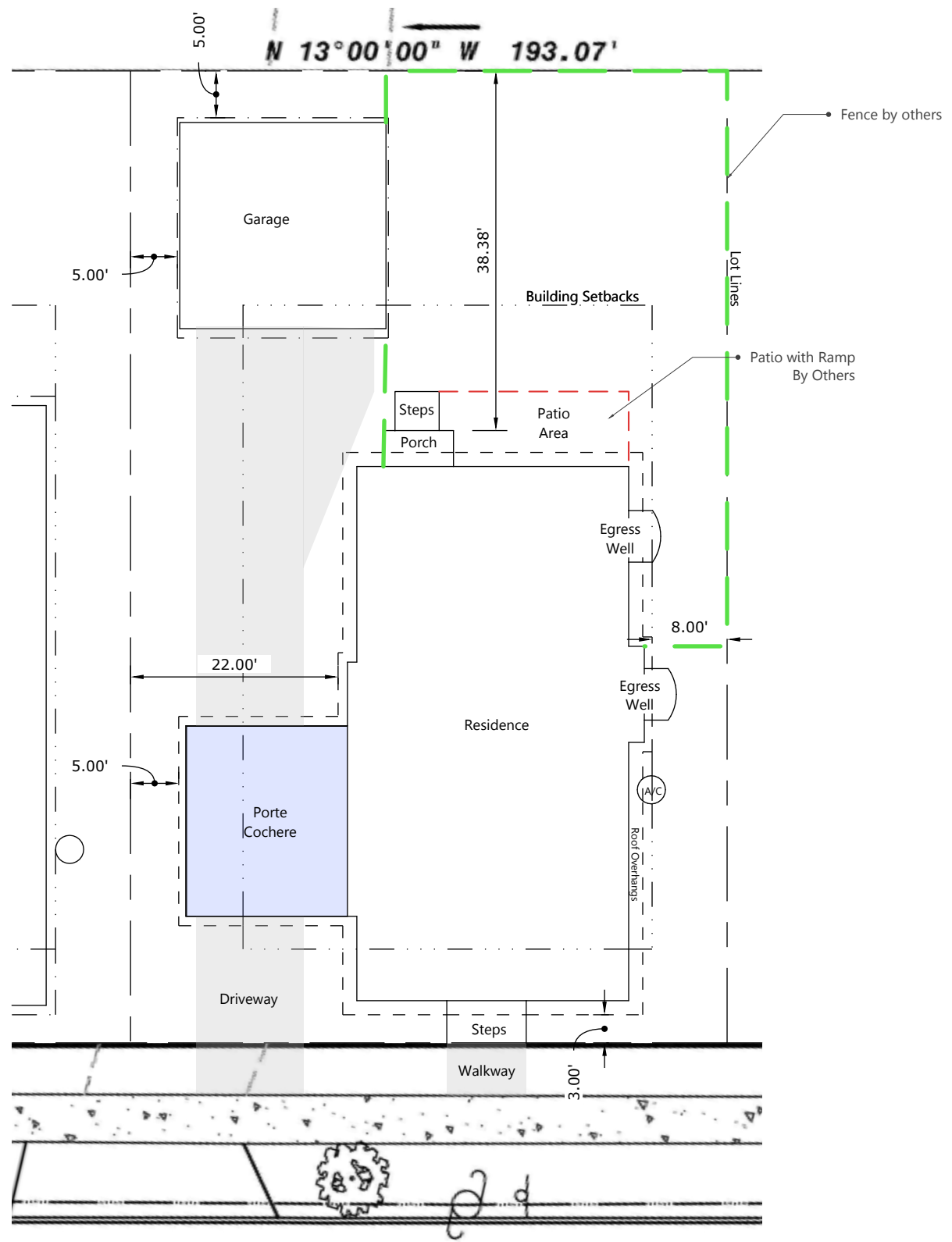
Plot Plan Scale: 1/16" = 1'-0"
